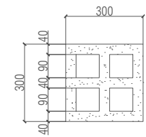
PLAN SCALE 1:20
